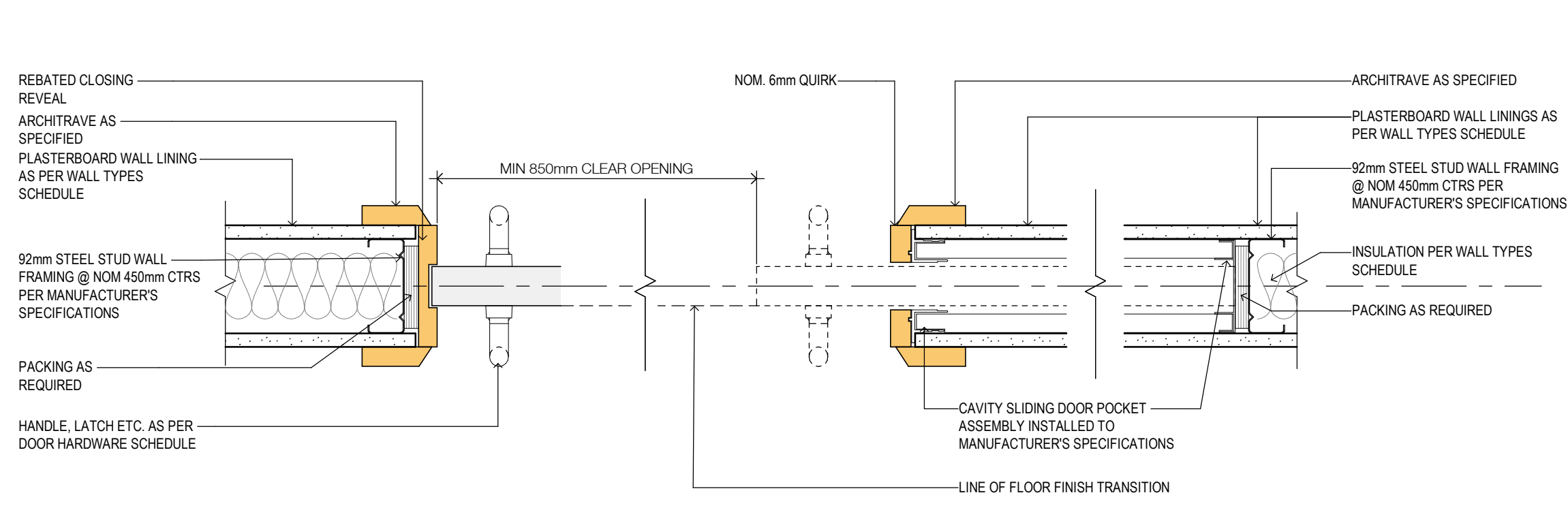
6 TYPICAL INTERNAL SLIDING DOOR PLAN DETAIL Scale 1:5
