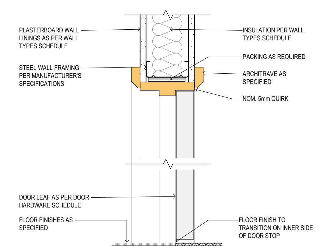
4 TYPICAL SWING DOOR HEAD DETAIL Scale 1:5
