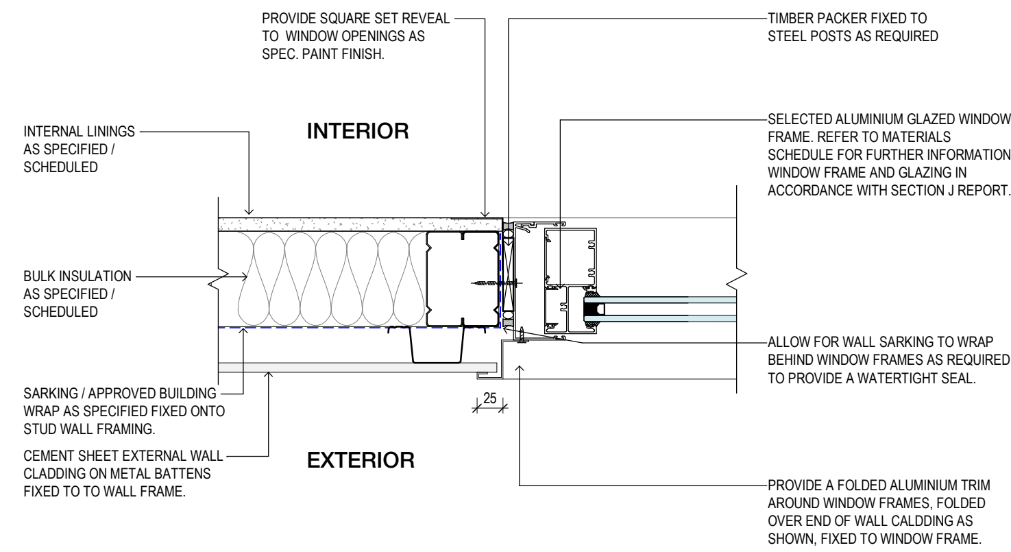
3 TYPICAL - GENERAL WINDOW JAMB - LIGHTWEIGHT WALL CLADDING Scale 1:5
