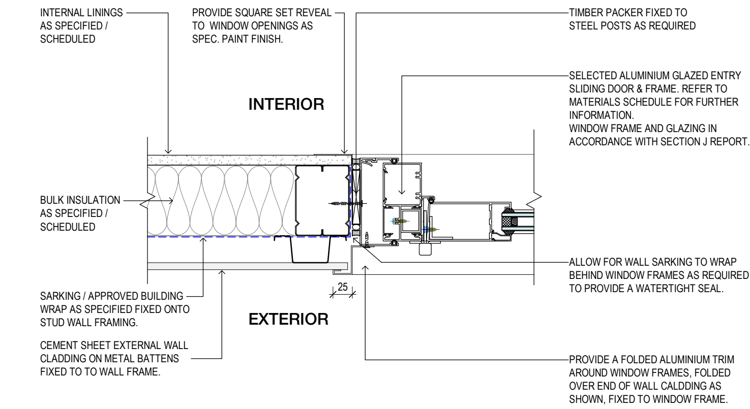
1 TYPICAL - EXTERNAL DOOR JAMB DETAIL - LIGHTWEIGHT WALL CLADDING Scale 1:5
