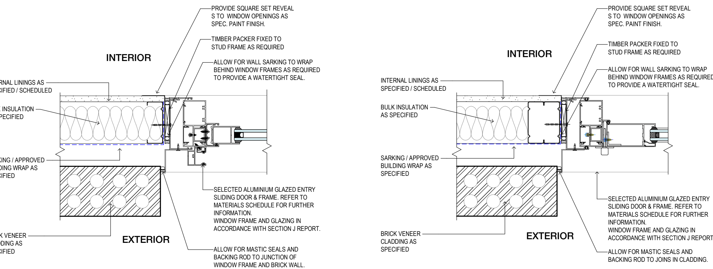
8 EXTERNAL SLIDING DOOR JAMB PLAN DETAIL Scale 1:5
