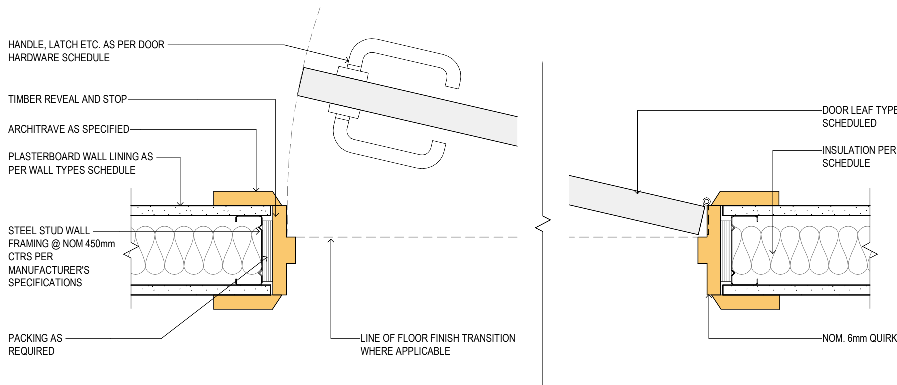
5 TYPICAL SWING DOOR JAMB DETAIL Scale 1:5
