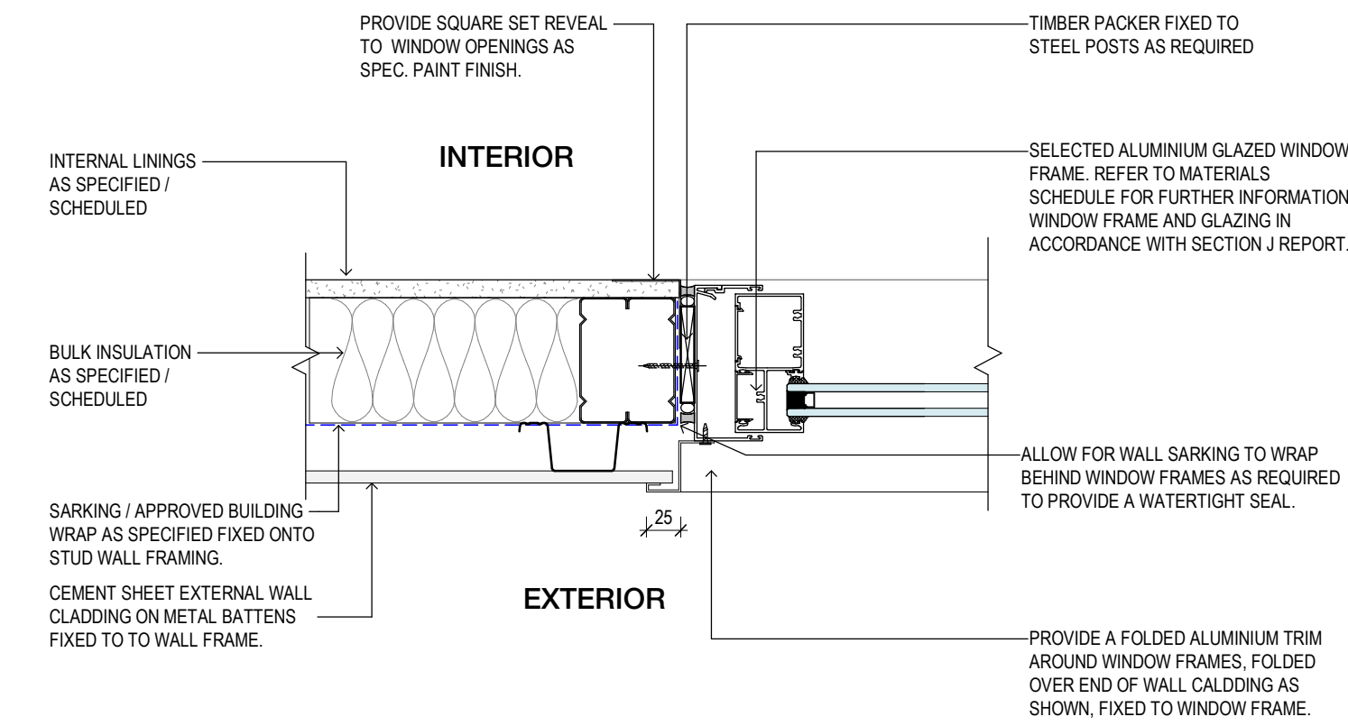
2 TYPICAL - SOU WINDOW JAMB - LIGHTWEIGHT WALL CLADDING Scale 1:5
