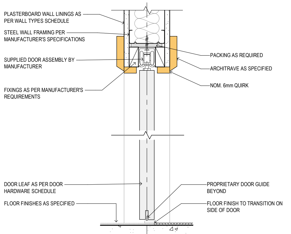
7 INTERNAL CAVITY SLIDING DOOR SILL & HEAD DETAIL Scale 1:5
